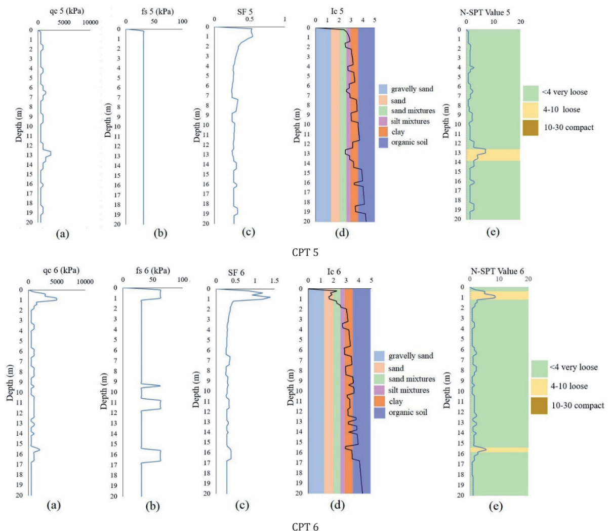
Figure 13. Liquefaction analysis at the sixth CPT testing location, illustrating (a) q_c vs depth, (b) f_s vs depth, (c) safety factor (SF) vs depth, (d) soil behavior type index vs depth, and (e) N-SPT Value vs depth.
