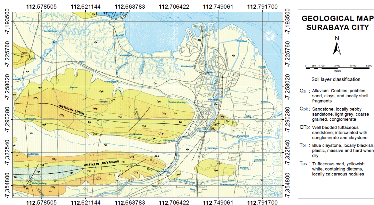
Figure 1 Geological map and coordinates of Surabaya City.
