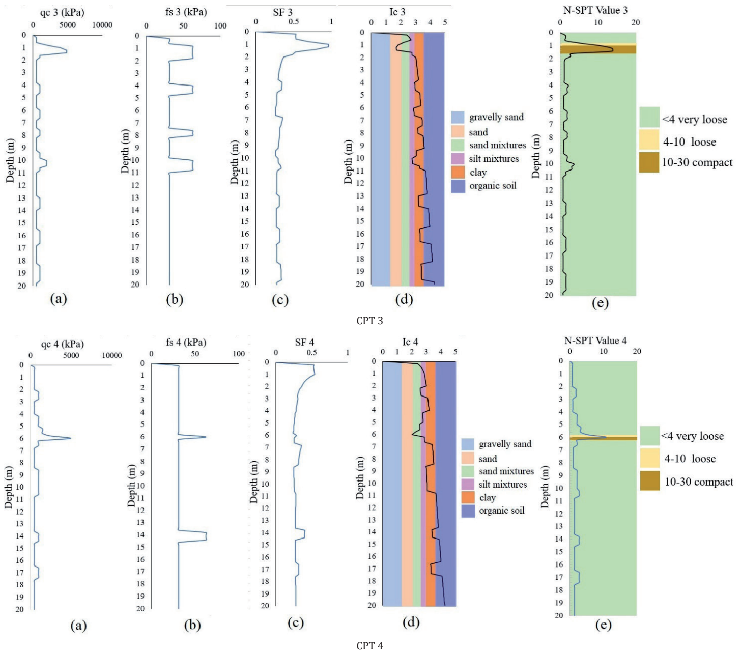
Figure 12. Liquefaction analysis at the third and the fourth CPT testing location, illustrating (a) q_c vs depth, (b) f_s vs depth, (c) safety factor (SF) vs depth, (d) soil behavior type index vs depth, and (e) N-SPT Value vs depth.
